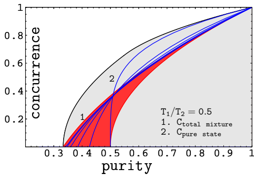
FIG. 4: (Color online) We present evolutions of the concurrence and the purity for the homogenization process in the case with the ratio of characteristic times T_1 and T_2 taking the constant value T_1/T_2 = 1/2 while the fixed point of the evolution varies from total mixture (unital process) to a pure state (non-unital process). In particular, when the fixed point of the homogenization is a total mixture then the homogenization dynamics in the C-P diagram is described by the line (1). This line lies below the line C_W with the final point C = 0 having the smallest value of the purity. On the other hand, when the fixed point of the evolution is a pure state, then the corresponding C-P line (2) ends in the point C = 0 with the largest value of the purity P = 1/2 .
