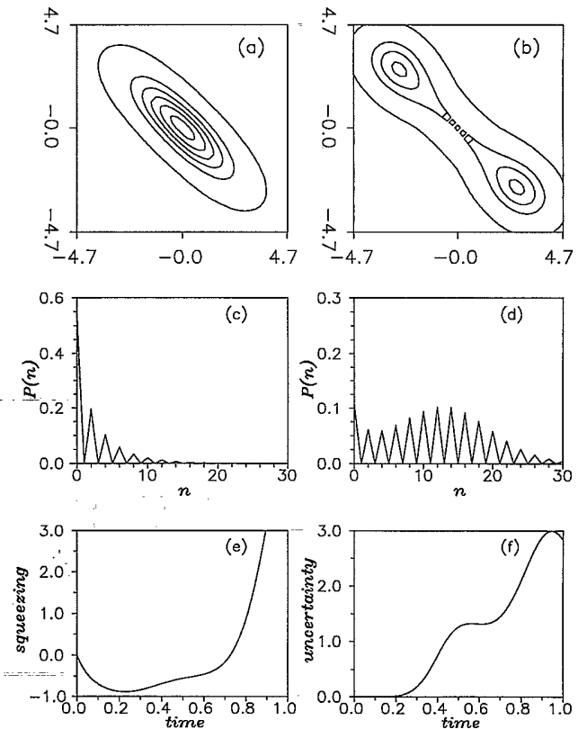
FIG. 2. Parameters of the a mode for two-photon down-conversion ( \beta=3 ): (a) Q function for \lambda_2 t=0.2 ; (b) Q function for \lambda_2 t=0.5 ; (c) photon-number distribution for \lambda_2 t=0.2 ; (d) for \lambda_2 t=0.5 ; (e) shows the time evolution of the squeezing parameter S_a^2 ; and (f) gives the uncertainty function u_a .
