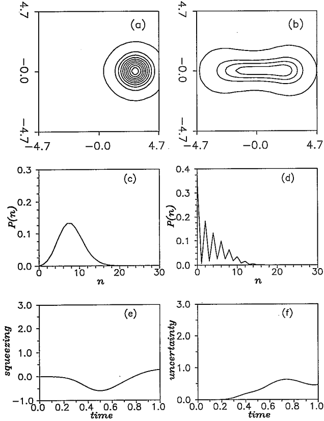
FIG. 3. The same parameters as in Fig. 2 but for the pump mode.
