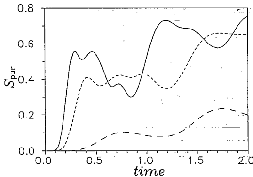
FIG. 1. The time evolution of the purity parameter S_{\text{pur}} in the two-photon down-conversion for initial state |0\rangle_a |\beta\rangle_b with \beta=1 (long-dashed curve), \beta=3 (short-dashed curve), and \beta=5 (solid curve). Increase of the intensity of the b mode leads to the stronger entanglement between the pump and the signal. Time scale is given by \lambda_2 t .
