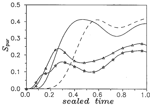
FIG. 7. The time evolution of the purity parameter S_{\text{pur}} in the k -photon down-conversions with \beta=3 : k=2 (dashed curve), k=3 (solid curve), k=4 (curve with \triangle ), k=5 (curve with \star ). The scaled time is taken to be \tau = t\sqrt{k!}\lambda_k .
