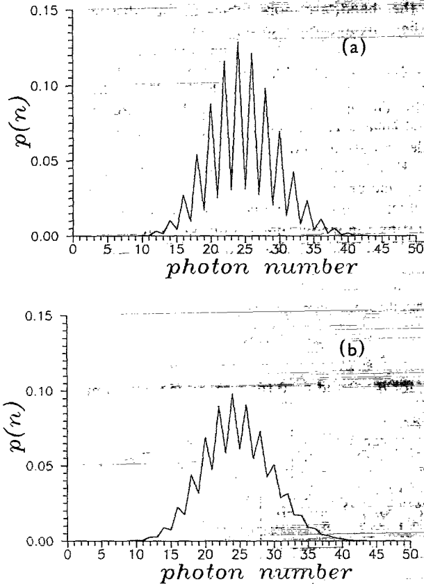
FIG. 5. The photon-number distribution \lambda(l, t) at \gamma t = 0.01 of the field mode initially prepared in the even CS ( \zeta = 5 ). The field mode interacts with a zero-temperature heat bath (a) and with a nonzero-temperature heat bath with \bar{n} = 1 (b). We see that the oscillations of the PND are much more visible when the field mode interacts with the zero-temperature heat bath.
