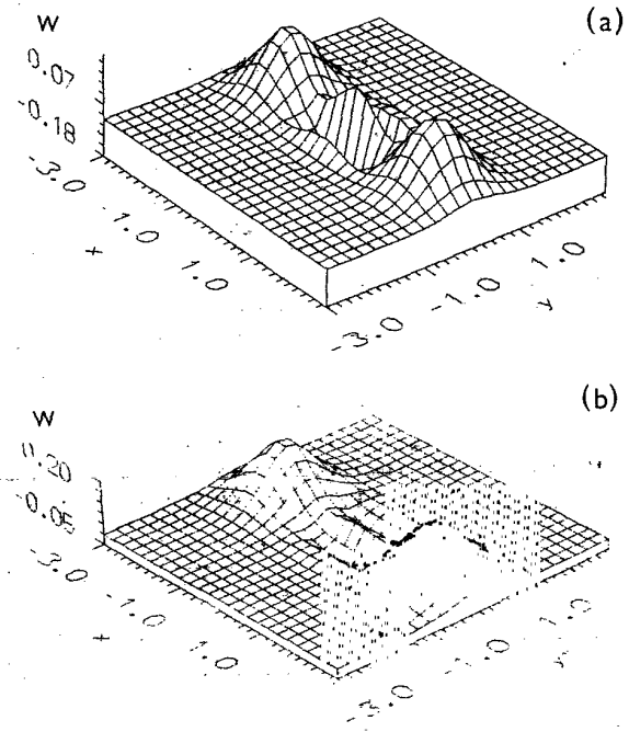
FIG. 2. The Wigner function at \gamma t = 0.1 of the field mode initially prepared in the even CS with \xi = 2 . The field mode interacts (a) with a zero-temperature heat bath ( \bar{n} = 0 ) and (b) with a nonzero-temperature heat bath ( \bar{n} = 1 ). We see that the interference term in the latter case ( \bar{n} \neq 0 ) is much more suppressed than the former case of zero temperature ( \bar{n} = 0 ).
