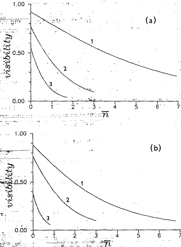
FIG. 6. The visibility of the field mode initially prepared in the even CS is plotted as a function of \bar{n} . In (a) we plot the visibility at \gamma t = 0.01 and \zeta = 3 (line 1); \zeta = 5 (line 2), and \zeta = 7 (line 3). We can easily see the decrease of the visibility with increasing of \zeta . In (b) we plot the visibility for a fixed value of \zeta = 5 and various values of \gamma t . In particular, line 1 corresponds to \gamma t = 0.005 , line 2 is for \gamma t = 0.01 , and line 3 is for \gamma t = 0.03 . The suppression of the visibility with increasing of the interaction (measurement) time is obvious.
