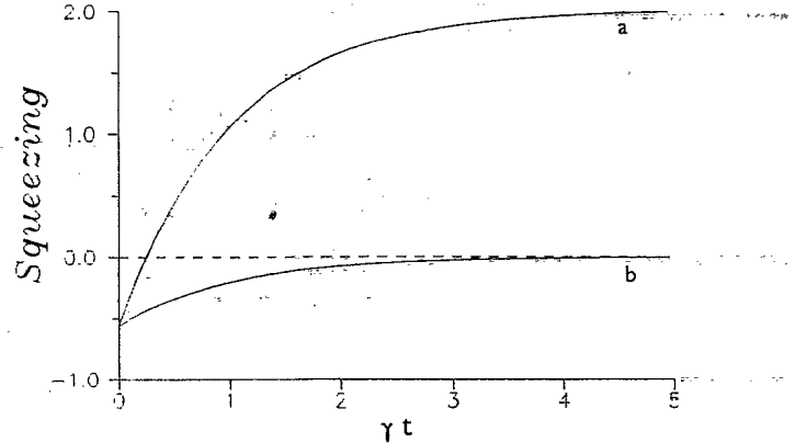
FIG. 4. The time evolution of the squeezing parameter S_2^{(2)} of the field mode initially prepared in the even CS ( \xi=0.8 ). The value of \xi has been chosen to optimize the squeezing at the initial time t=0 . Line (b) corresponds to the interaction with a zero-temperature heat bath ( \bar{n}=0 ) while line (a) describes the time evolution of squeezing when the field mode is coupled to a nonzero-temperature heat bath ( \bar{n}=1 ).
