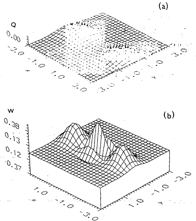
FIG. 1. The Q function (a) and the Wigner function (b) for the even CS with \xi=2 . We see that the quantum-interference term is more visible in the Wigner function but not in the Q function [ x = \text{Re}(\alpha) and y = \text{Im}(\alpha) ].
