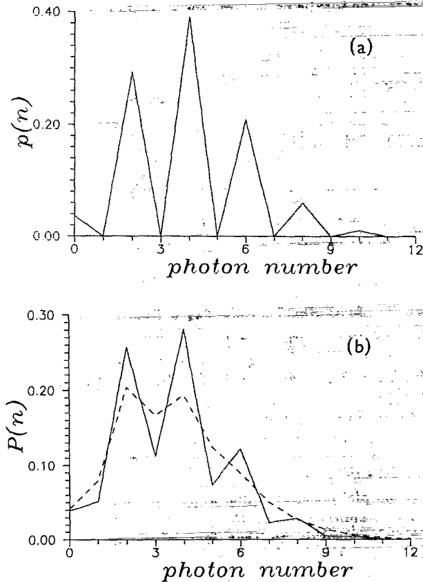
FIG. 3. (a) The photon-number distribution \mathcal{A}(l, 0) for the initial even CS with \xi=2 (a). We see typical oscillations emerging from the quantum-interference between component states of the even CS. (b) The photon-number distribution \mathcal{A}(l, t) at \gamma t = 0.01 of the field mode initially prepared in the even CS. The field mode interacts with a zero-temperature heat bath (solid line) and with a non-zero-temperature heat bath of \bar{n}=1 (dotted line). We see that the oscillations of the PND are much more pronounced in the case of the zero-temperature heat bath.
