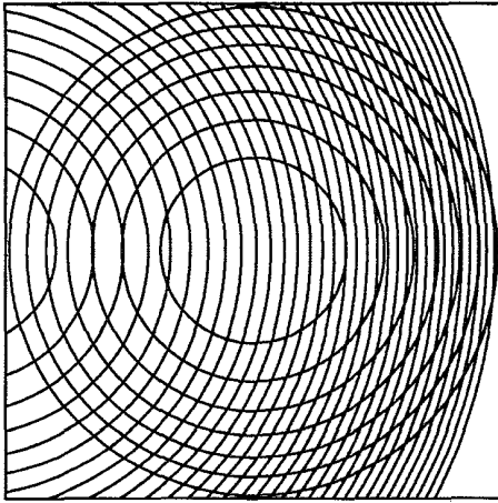
FIG. 4. Pictorial representation of number states and displaced number states in phase space.
