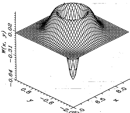
FIG. 2. Wigner function for the displaced number state |7, 1\rangle .
