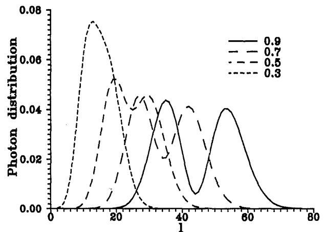
FIG. 5. Effect of dissipation, or, equivalently, of nonunity quantum efficiency \mu for the detection of the oscillations of the photon distribution for the displaced number state |7,1\rangle . We plot the photon distribution corresponding to \mu=0.9, 0.7, 0.5, 0.3 . The oscillations are still resolved for \mu=0.5 .
