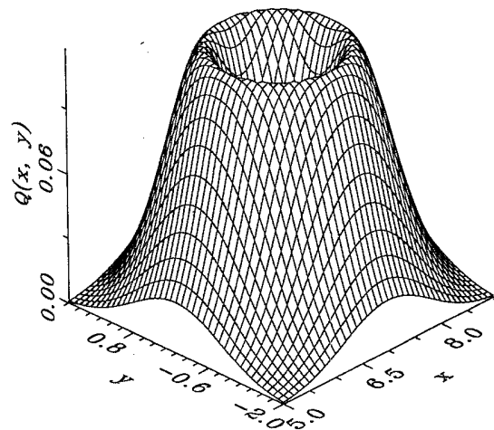
FIG. 1. Q function for the displaced number state |7, 1\rangle .
