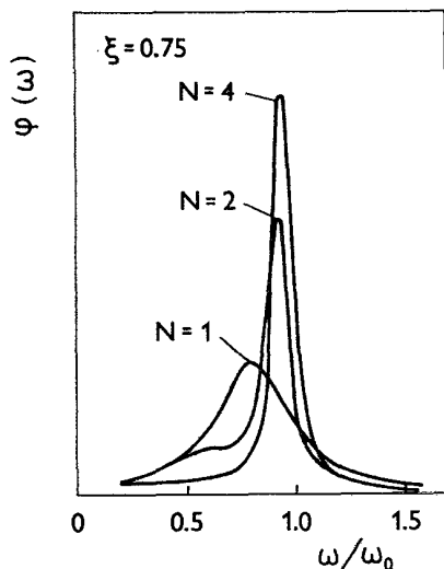
FIG. 1. Spectral line \phi(\omega) for N=1, 2, and 4 when \xi=0.75 and \Gamma=\Delta=0.2\omega_0 .
