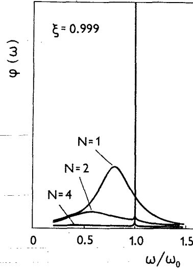
FIG. 2. Spectral line \phi(\omega) for N=1, 2, and 4 when \xi=0.999 and \Gamma=\Delta=0.2\omega_0 .
